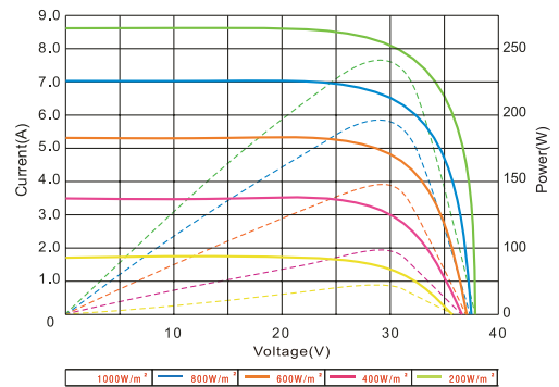
Electrical Performance (Cell Temperature: 25°C)
